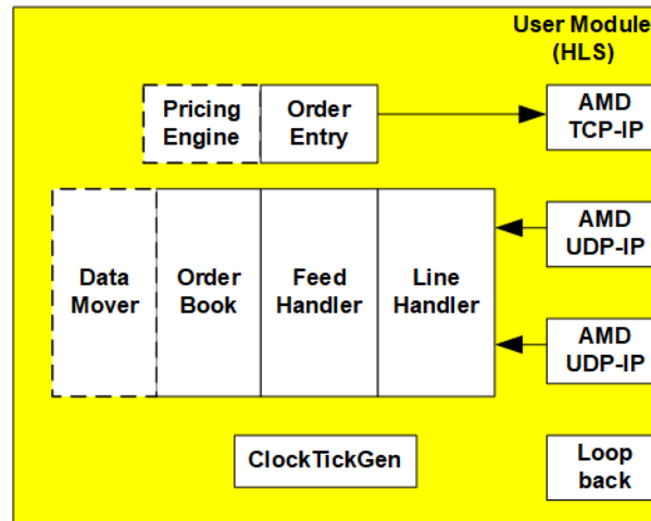
Figure 15 User Module Component
