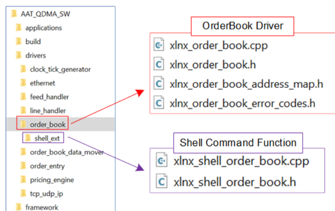
Figure 34 OrderBook Driver
