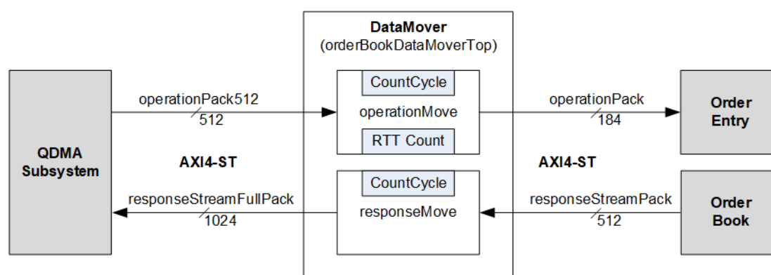
Figure 16 DataMover Submodule
