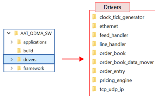
Figure 29 AAT-QDMA Driver
