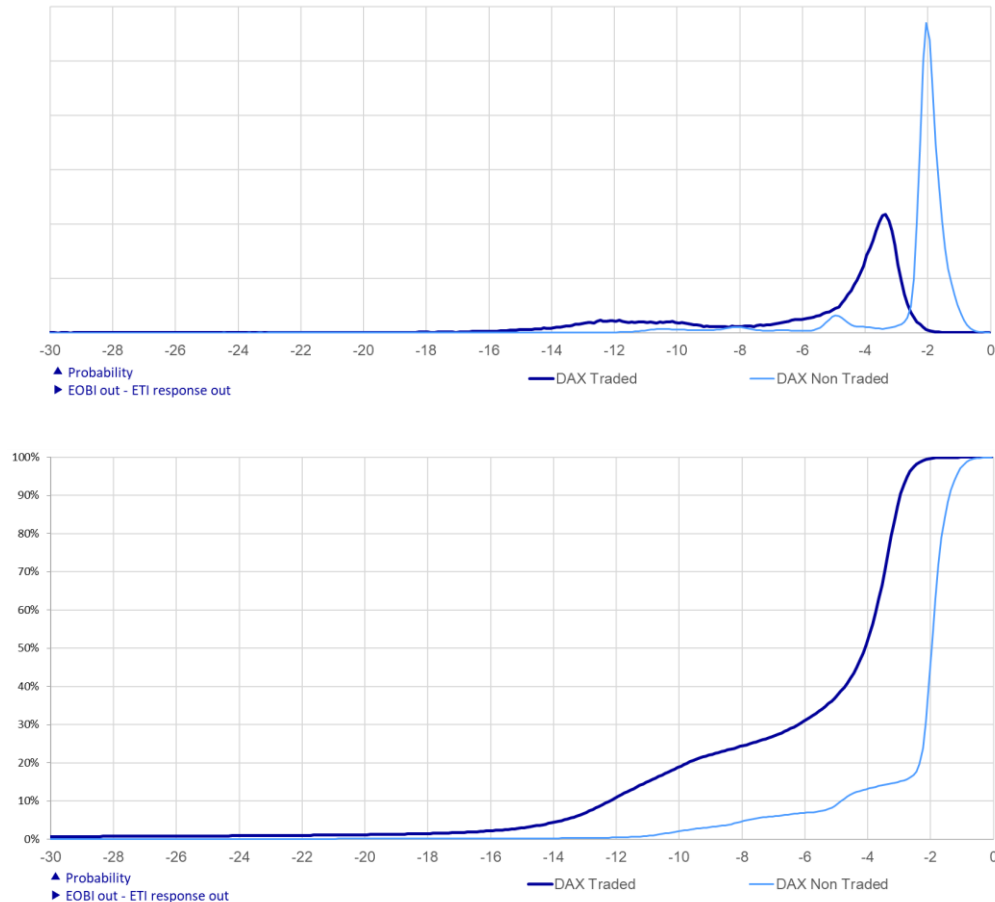
ETI vs EOBI for Xetra DAX 2025-02-13
