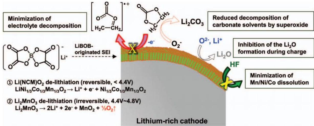
자료: Effect of Lithium Bis(oxalato)borate Additive on Electrochemical Performance of Li1.17Ni0.17Mn0.5Co0.17O2 Cathodes for Lithium-Ion Batteries (Sung Jun Lee et al 2014), 하이투자증권
