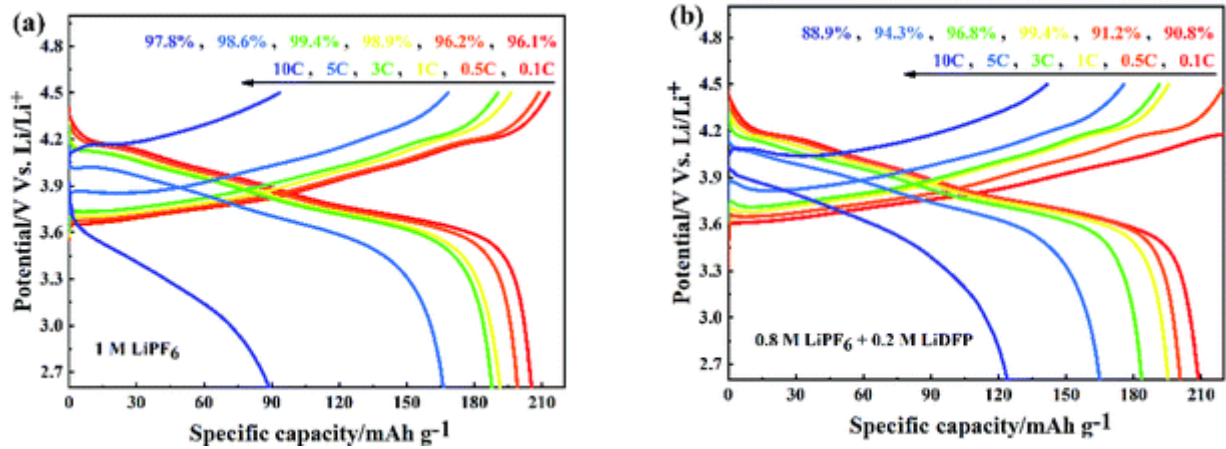
자료: A LiPO 2 F 2 /LiPF 6 dual-salt electrolyte enabled stable cycling performance of nickel-rich lithium ion batteries (Liu et al 2020), 하이투자증권
