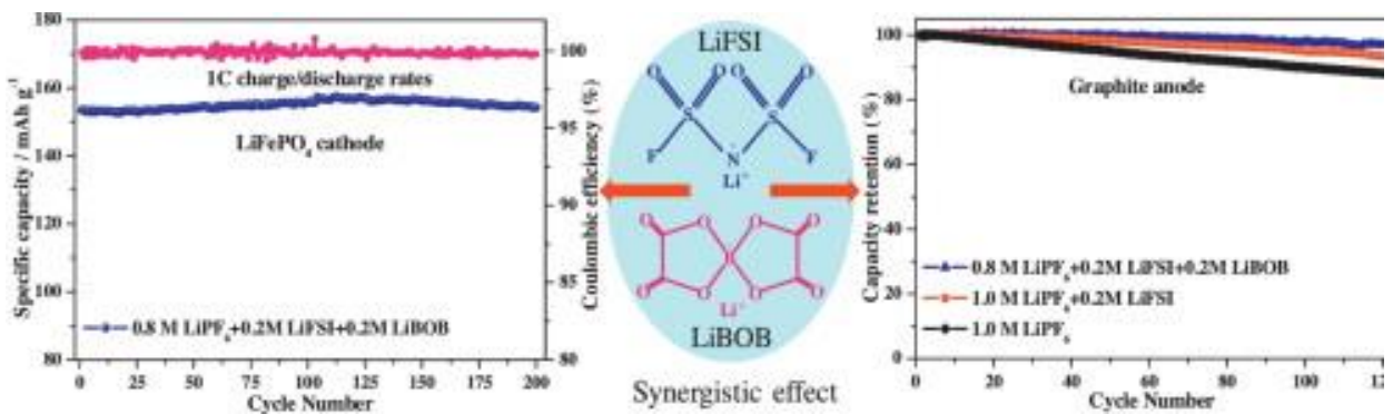
자료: Synergistic effect between lithium bis(fluorosulfonyl)imide (LiFSI) and lithium bis-oxalato borate (LiBOB) salts in LiPF 6 -based electrolyte for high-performance Li-ion batteries (Zhang et al 2014), 하이투자증권
