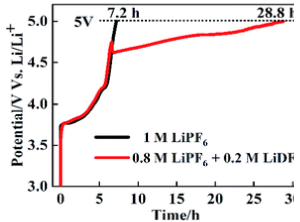
자료: A LiPO 2 F 2 /LiPF 6 dual-salt electrolyte enabled stable cycling performance of nickel-rich lithium ion batteries (Liu et al 2020), 하이투자증권
